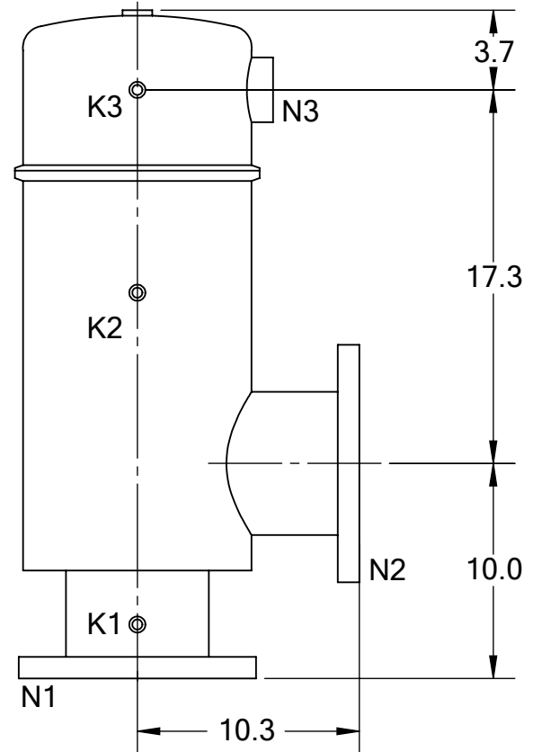
SIDE VIEW
