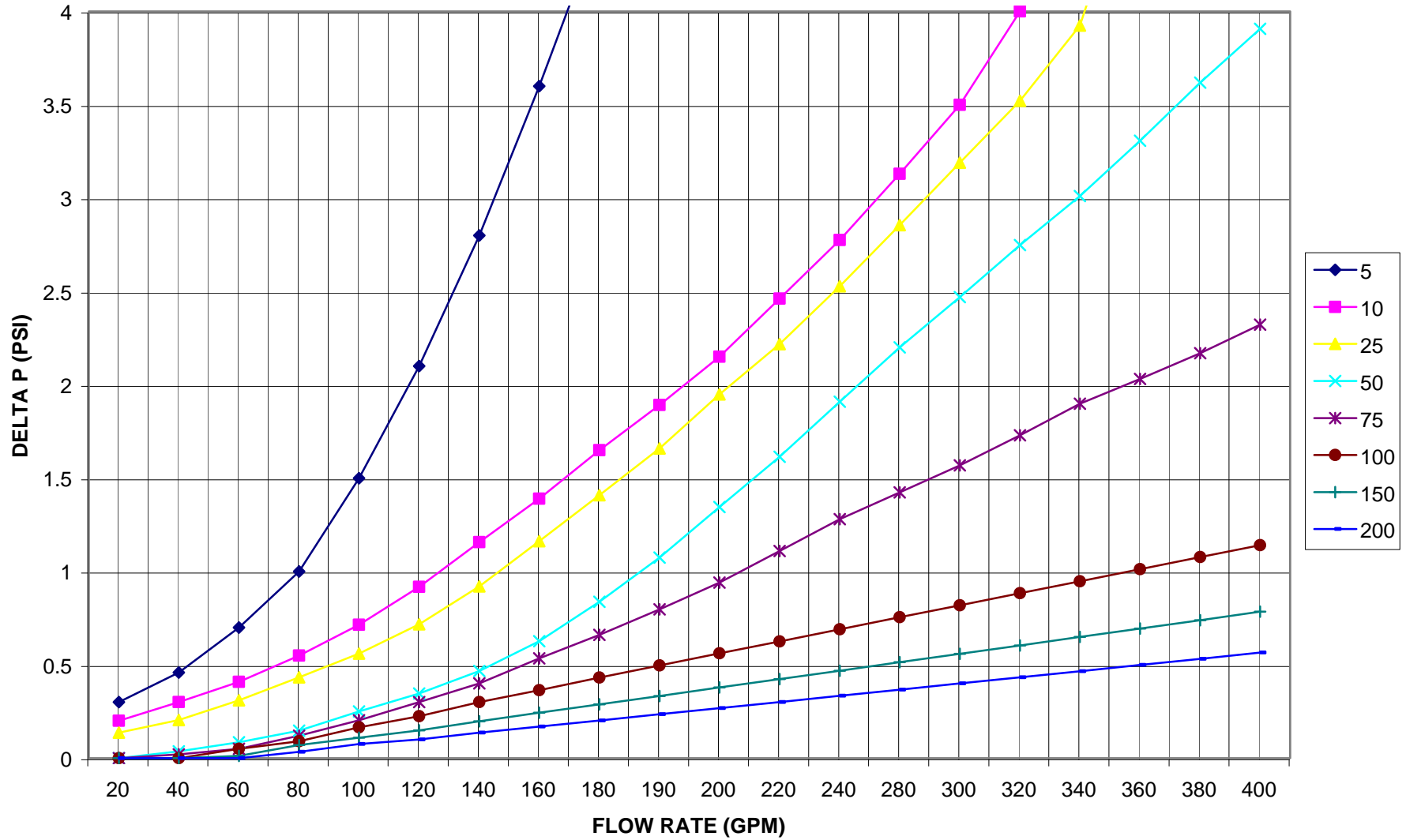
PRESSURE DROP DATA 1SQ FT.
